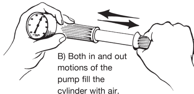
Figure 3. Hand pump operation
